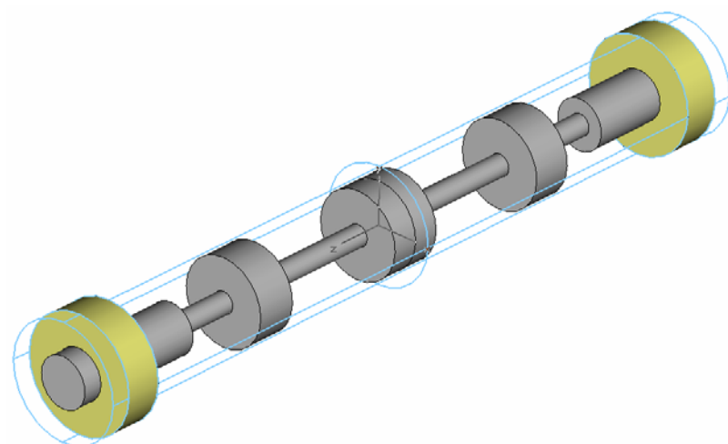
Abb. 2: Das CST MWS Modell.
