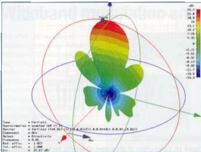
Figure 11: 3D far-field pattern of the directivity for simultaneous excitation, phase offsets are zero
