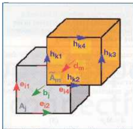
Figure 1: Allocation of the voltage and flux components in the mesh
