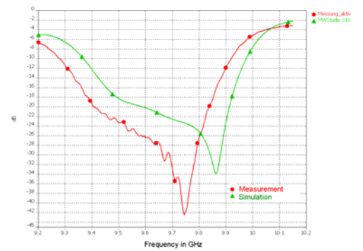
Fig.6: Comparison of the reflection parameter S11
