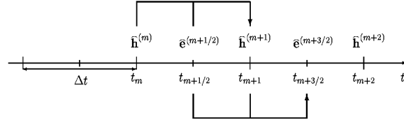
Fig. 2: The leap-frog scheme.
