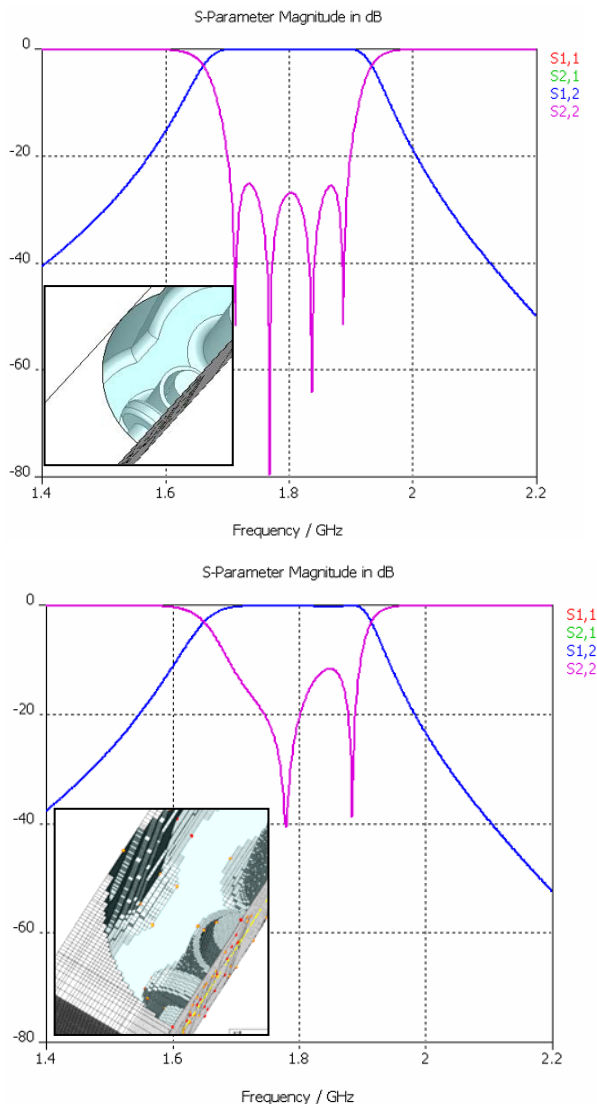
Fig.10. Simulated S-parameters for the 4-post pass-band filter. Upper plot: PBA mesh; lower plot: staircase mesh.
