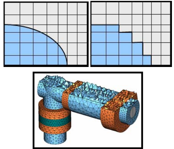
Fig. 2. Examples of PBA, staircase and tetrahedral meshes.
