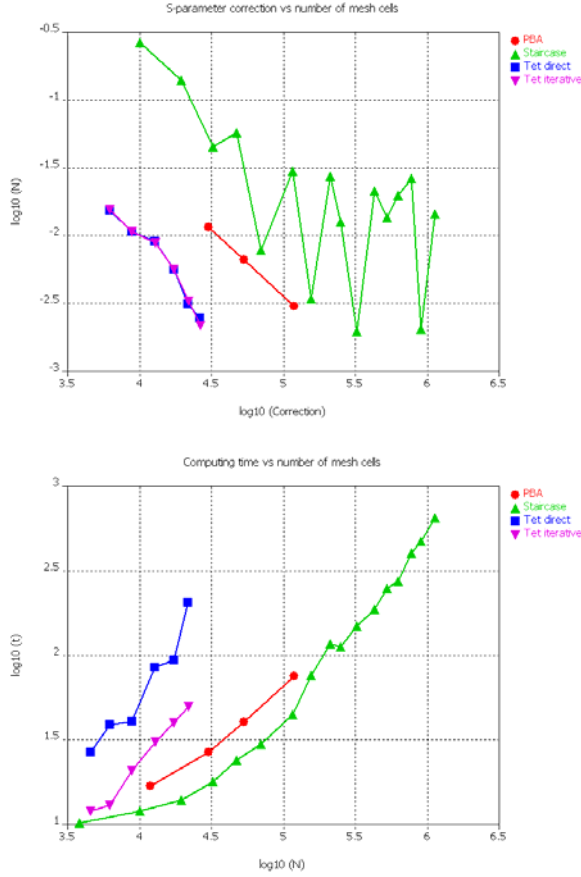
Fig. 6. Coaxial connector results. Upper plot: S-parameter correction vs number of mesh cells; Lower plot: computing time vs number of mesh cells
