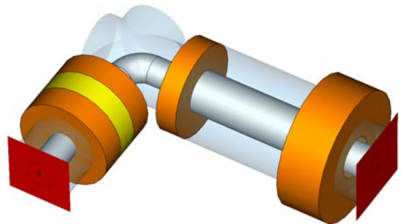
Fig. 5. Coaxial connector test structure.
