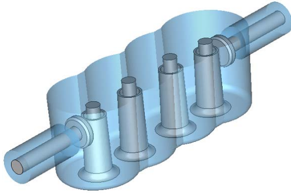
Fig. 9. 4-post pass-band filter. Model courtesy of the company Spinner GmbH, Westerham, Germany.
