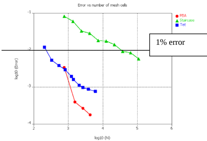
Fig. 3. Error of the line impedance of a coaxial cable vs the number of mesh cells.
