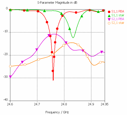
Fig. 8. Simulated S-parameters of the 16-port power divider, for PBA and staircase meshes
