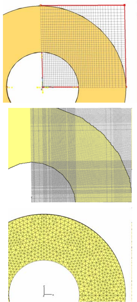
Fig. 4. Coaxial cable impedance simulation: Final mesh at the end of the convergence study, for PBA (4300 meshcells), staircase (110,000 meshcells) and tetrahedral (6175 meshcells) meshes.
