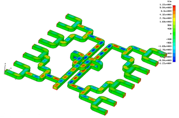
Fig. 7. 16-port power divider
